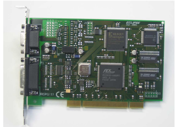
IRISPCI PCI 2 AXIS STEPPER MOTOR CONTROLLER
